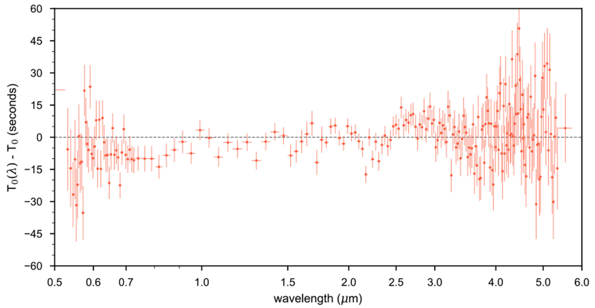
Extended Data Fig. 3 | The wavelength-dependent central transit time in seconds. Structure is apparent—the prominent water and carbon dioxide absorption features at 2.7 μm and 4.2 μm, respectively, appear to arrive ~20 s
